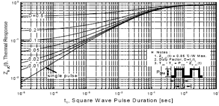
Figure 11-1. Transient Thermal Response Curve for OSP8N65C
