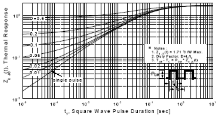
Figure 11-1. Transient Thermal Response Curve for OSP730C
