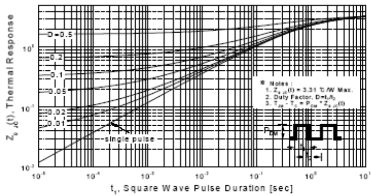
Figure 11-2. Transient Thermal Response Curve for OSF730C
