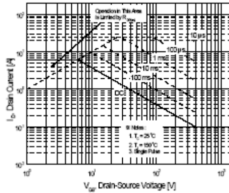
Figure 9-2. Maximum Safe Operating Area for OSF730C
