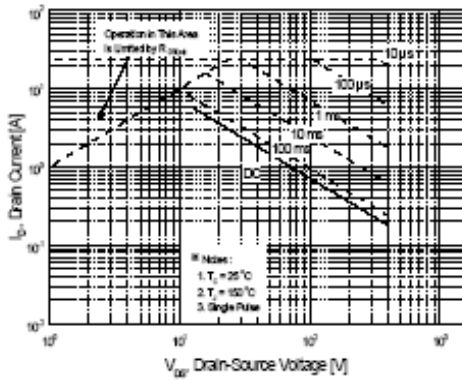
Figure 9-1. Maximum Safe Operating Area for OSP730C
