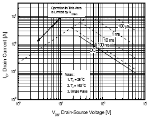
Figure 9-1. Maximum Safe Operating Area for OSP2N60C
