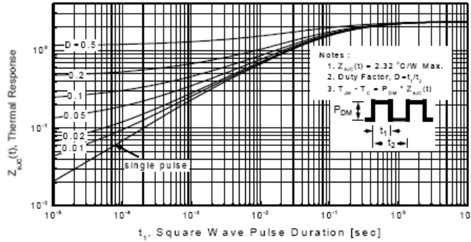
Figure 11-1. Transient Thermal Response Curve for OSP2N60C
