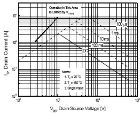
Figure 9-2. Maximum Safe Operating Area for OSF2N60C
