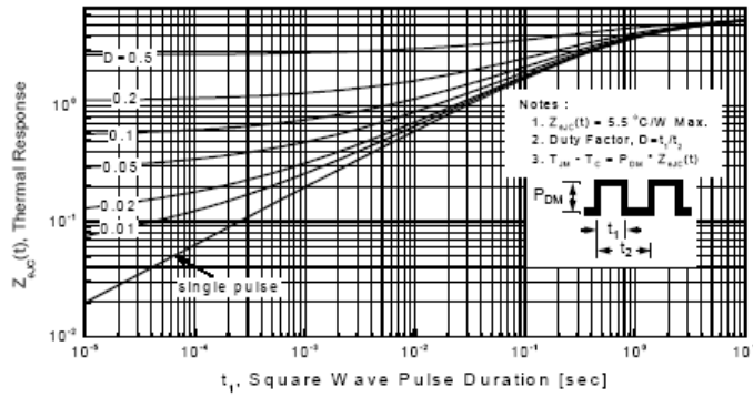
Figure 11-2. Transient Thermal Response Curve for OSF2N60C
